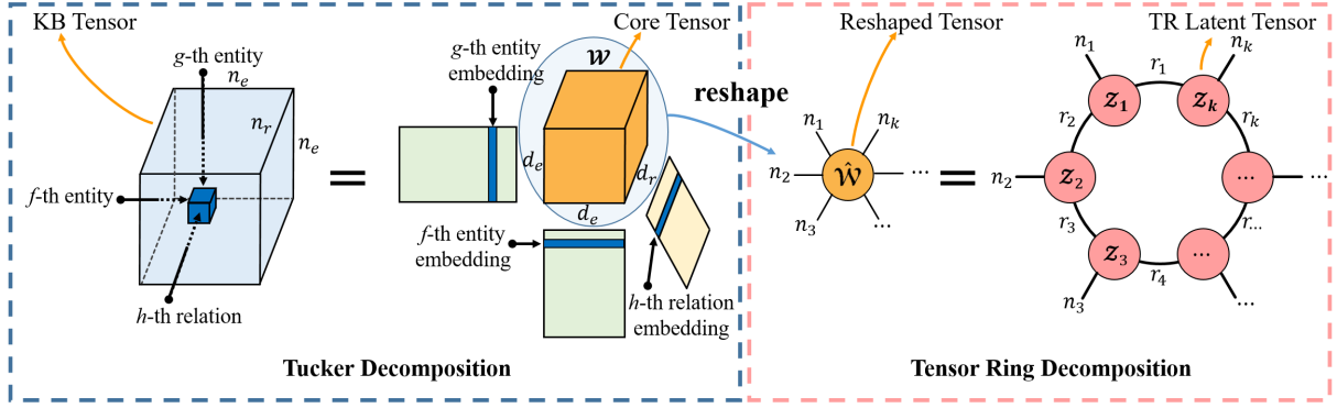
Figure 1: The main framework of GETD model.
