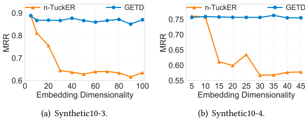
Figure 3: MRR for n-Tucker and GETD for different embeddings sizes. Evaluated on Synthetic10-3 (left) and Synthetic10-4 (right).
