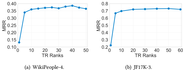
Figure 5: MRR of GETD on WikiPeople-4 (left) and JF17K-3 (right) under different TR-ranks.
