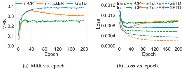
Figure 2: Overfitting in n-Tucker observed from MRR (left) and loss (right). Evaluated on WikiPeople-4.
