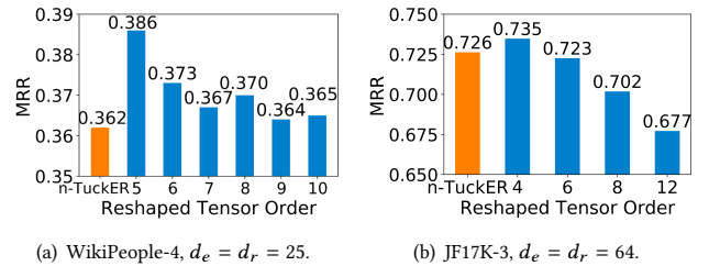
Figure 6: MRR of GETD on WikiPeople-4 (left) and JF17K-3 (right) under different reshaped tensor orders.
