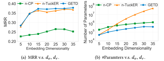
Figure 4: MRR (left) and number of parameters (right) under different embedding sizes. Evaluated on WikiPeople-4.
